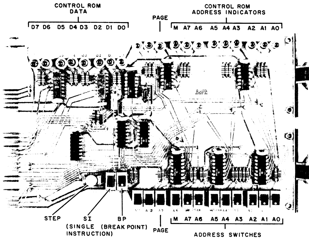
Figure 5-4 Service Module M7335
