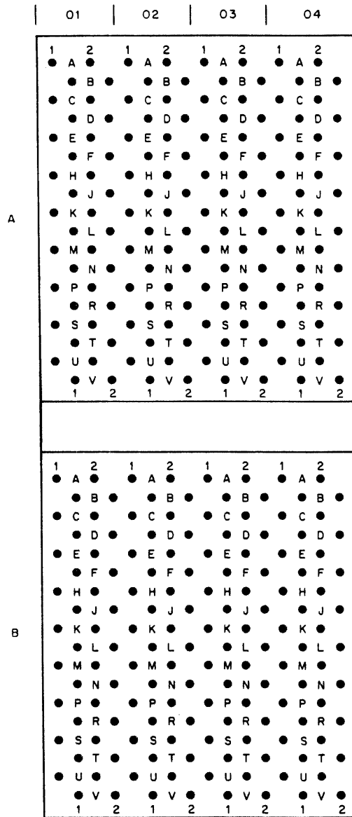
Figure 2 H803 Connector Block, Pin Assignments
