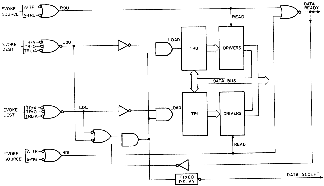
Figure 4-17 Transfer Register
