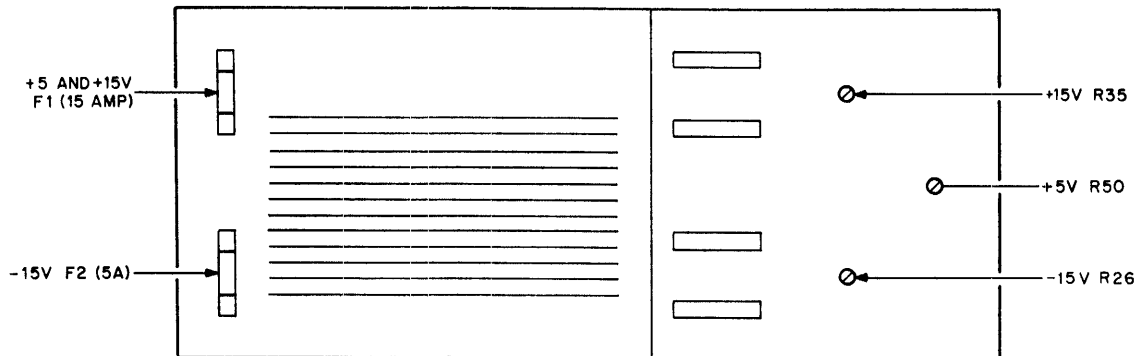
Figure 5-9 H740 Power Supply Fuses and Adjustment Controls
