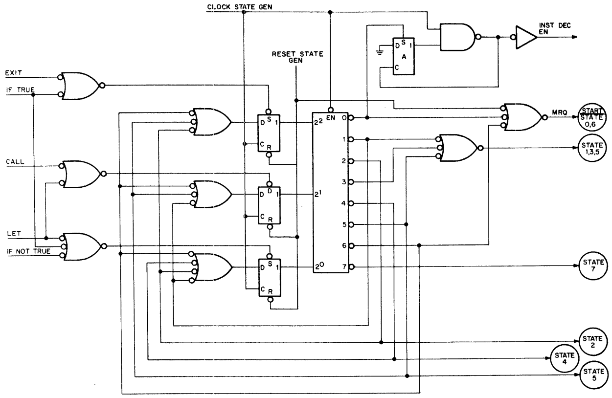
Figure 4-5 State Generator
