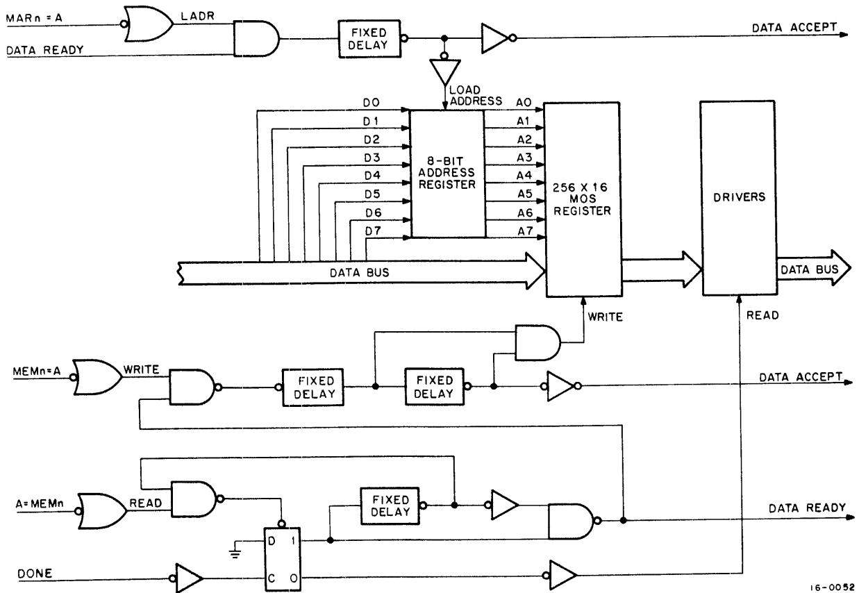
Figure 1 Data R/W MOS Memory Option MS16-D, Block Diagram
