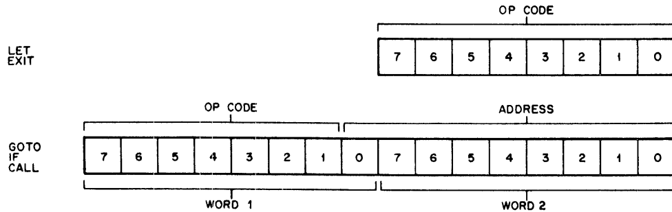
Figure 3-1 Instruction Format
