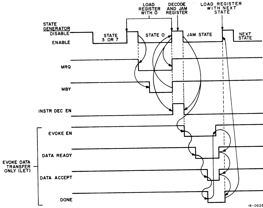
Figure 4-7 State Generator Timing Diagram
