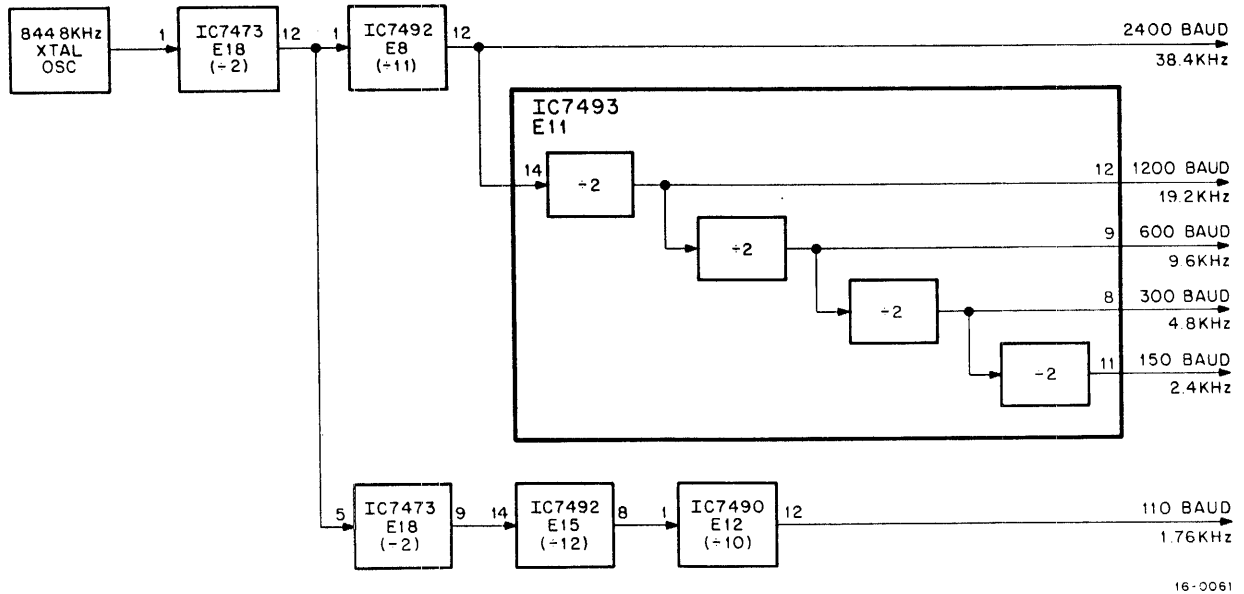
Figure 3 Clock Frequency Divider Chain, Block Diagram
