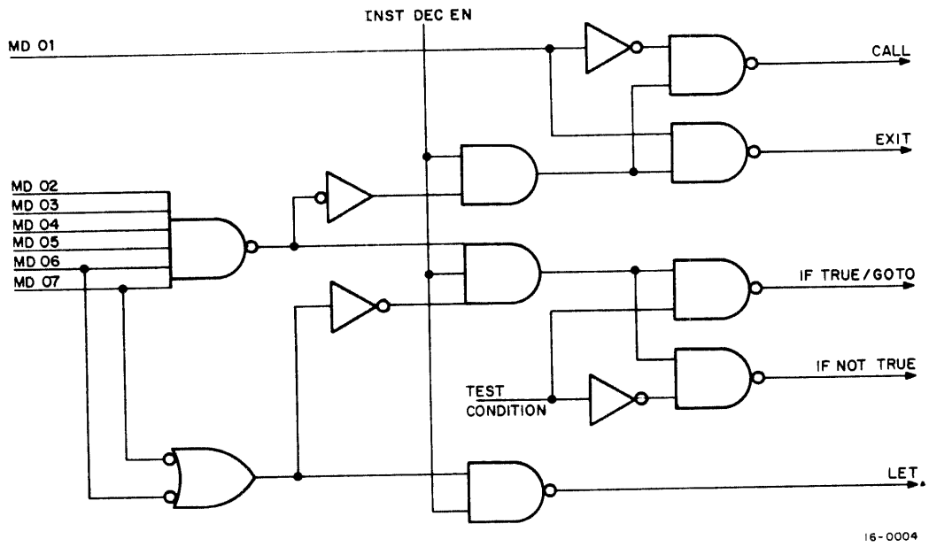
Figure 4-4 Instruction Decoder
