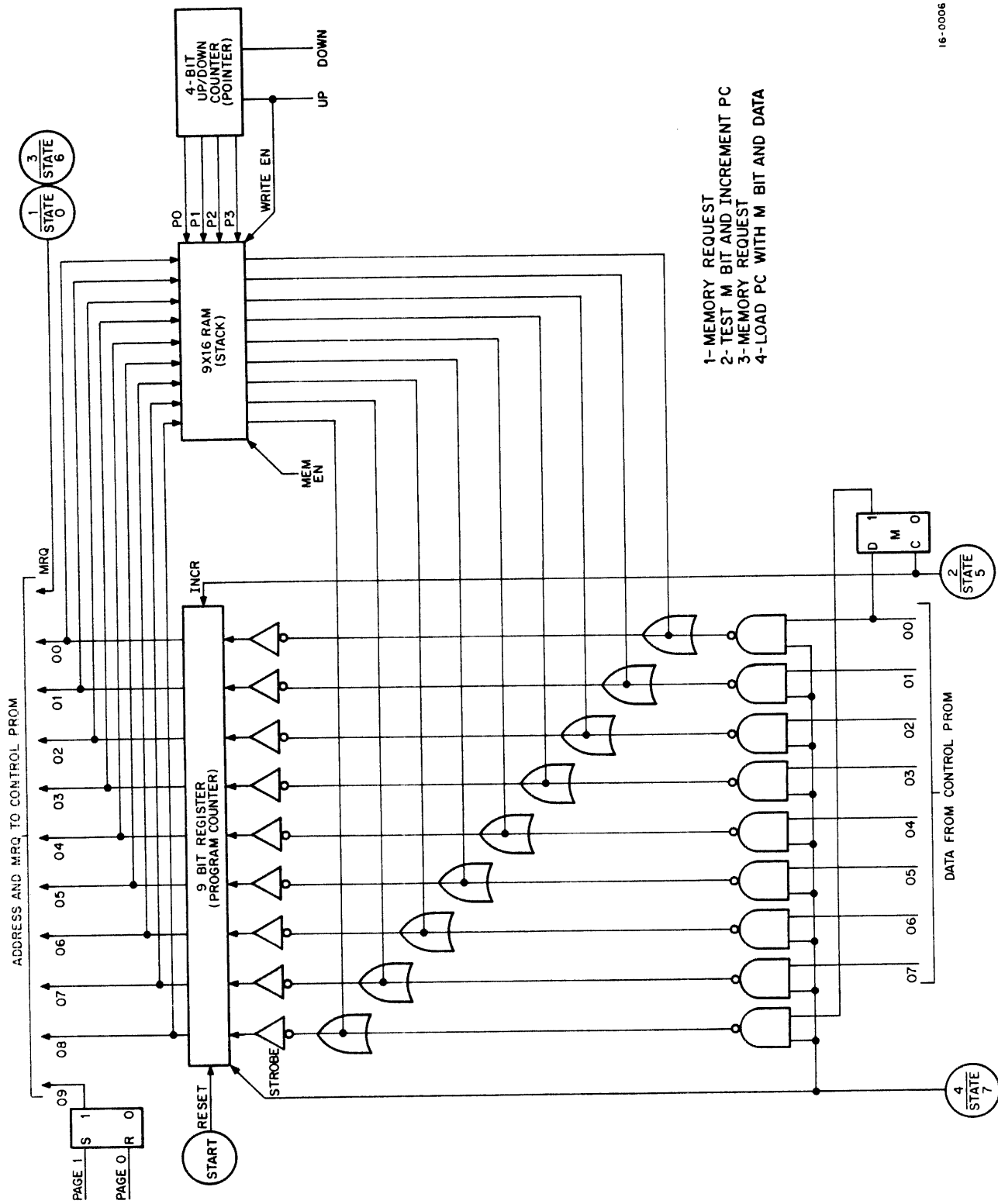
Figure 4-9 Program Counter and Stack - GOTO/IF (true) Instruction
