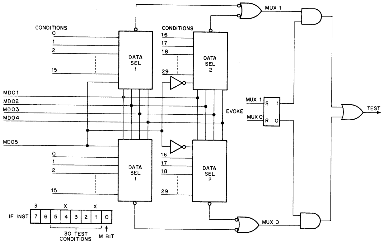
Figure 4-14 Boolean Multiplexers
