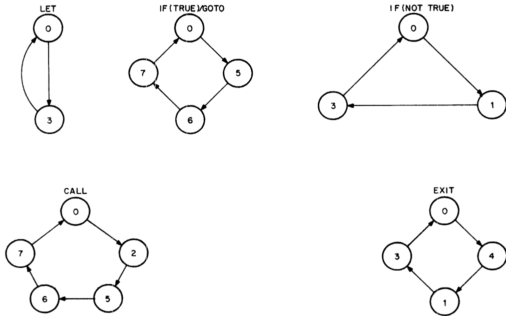
Figure 4-6 State Generator State Diagram
