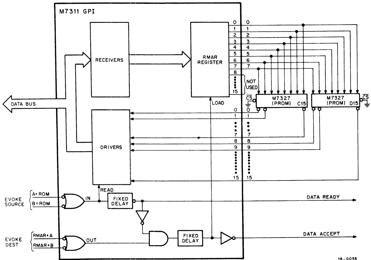
Figure 1 Data PROM Option MR16-E/F, Block Diagram
