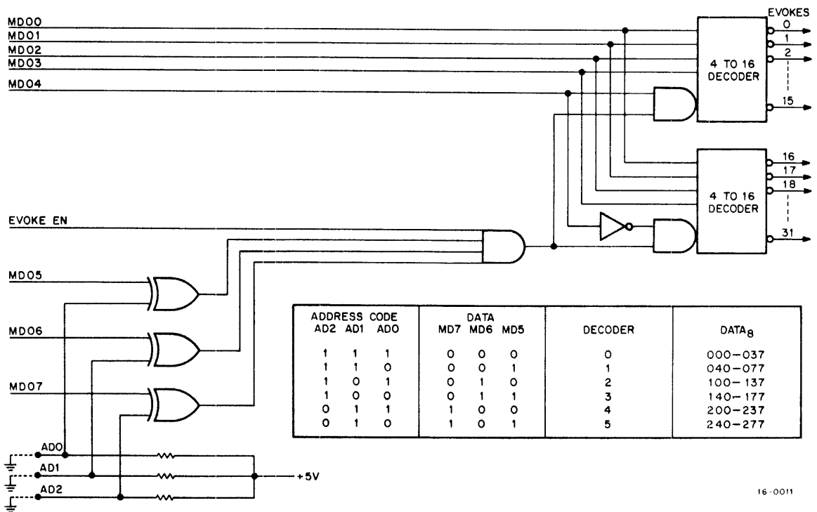
Figure 4-15 Evoke Decoder
