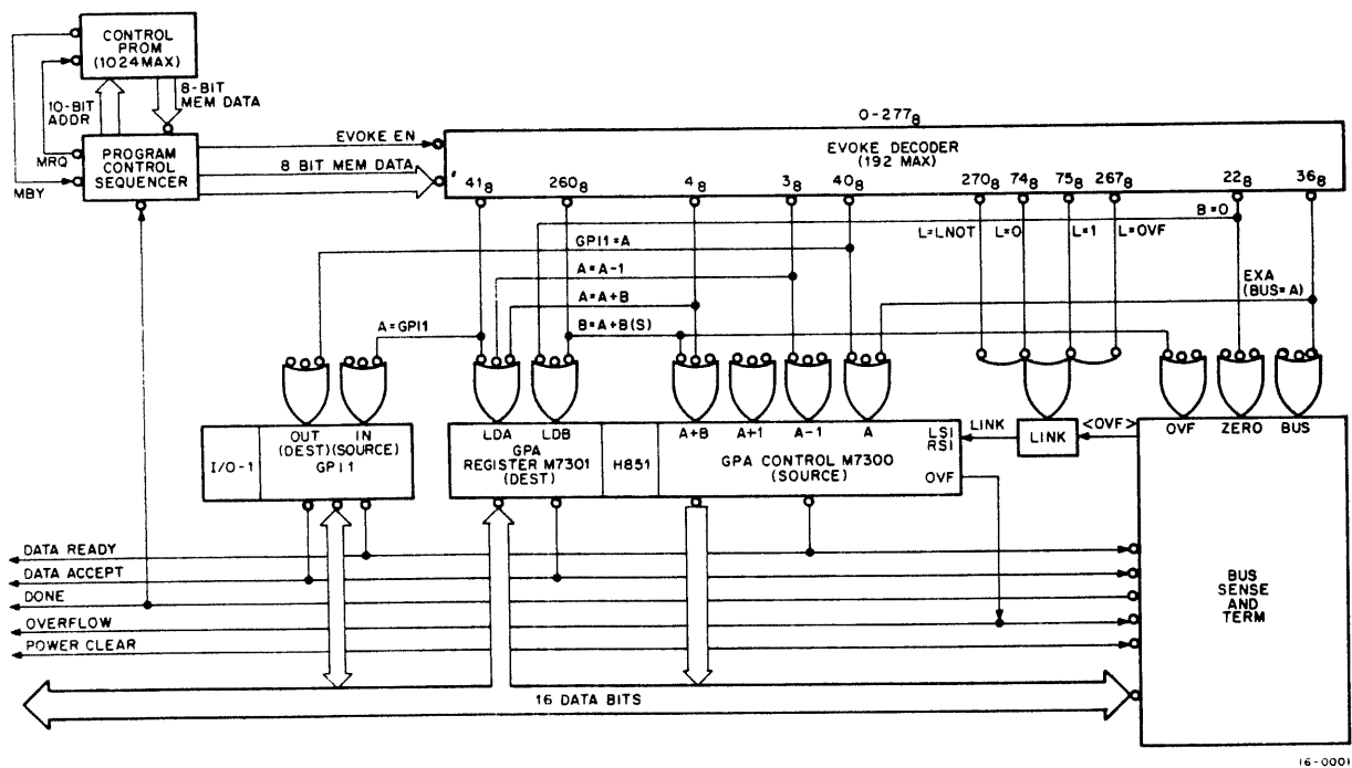
Figure 4-1 Evoke Data Transfer Scheme
