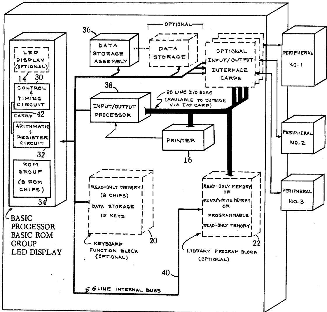
CALCULATOR BLOCK DIAGRAM
